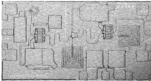
Figure 9. Photograph of IF Amplifier
