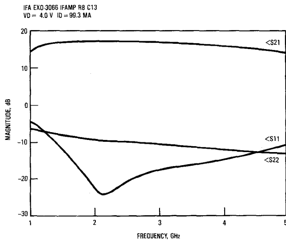
Figure 10. IF Amplifier Test Result
